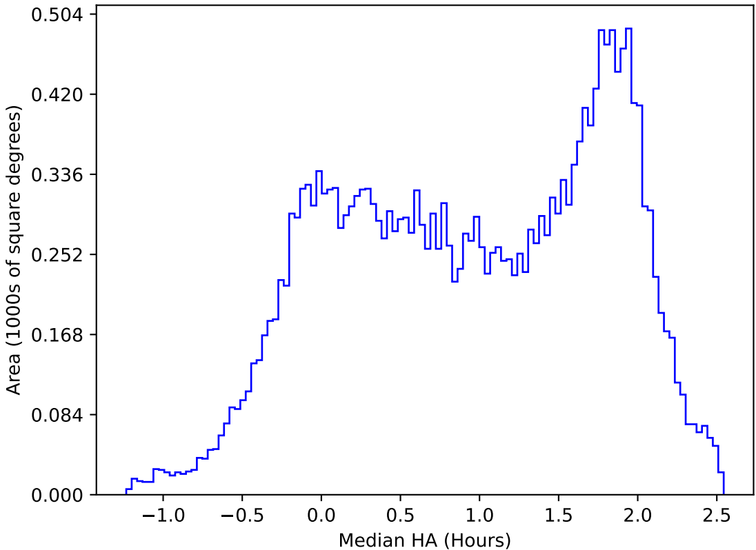
too_elab_heavy_r32_d3_griz_v3.4_10yrs All sky u band: Median HA
