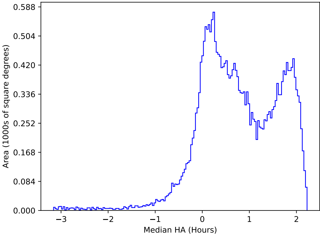
too_elab_heavy_r32_d3_griz_v3.4_10yrs All sky r band: Median HA
