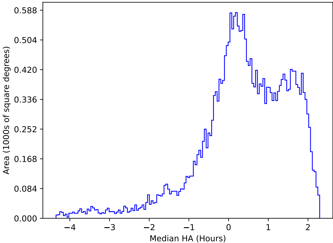
too_elab_heavy_r32_d3_griz_v3.4_10yrs All sky g band: Median HA
