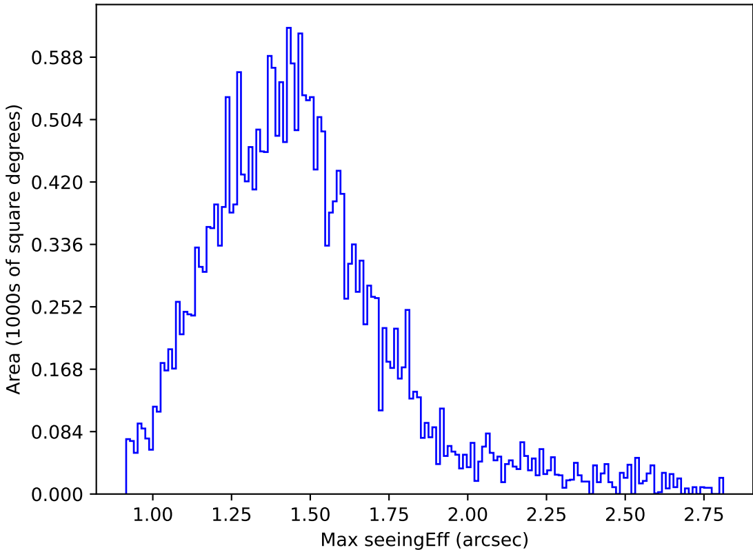
too_elab_heavy_r32_d3_griz_v3.4_10yrs Yr 1 z band: Max seeingEff
