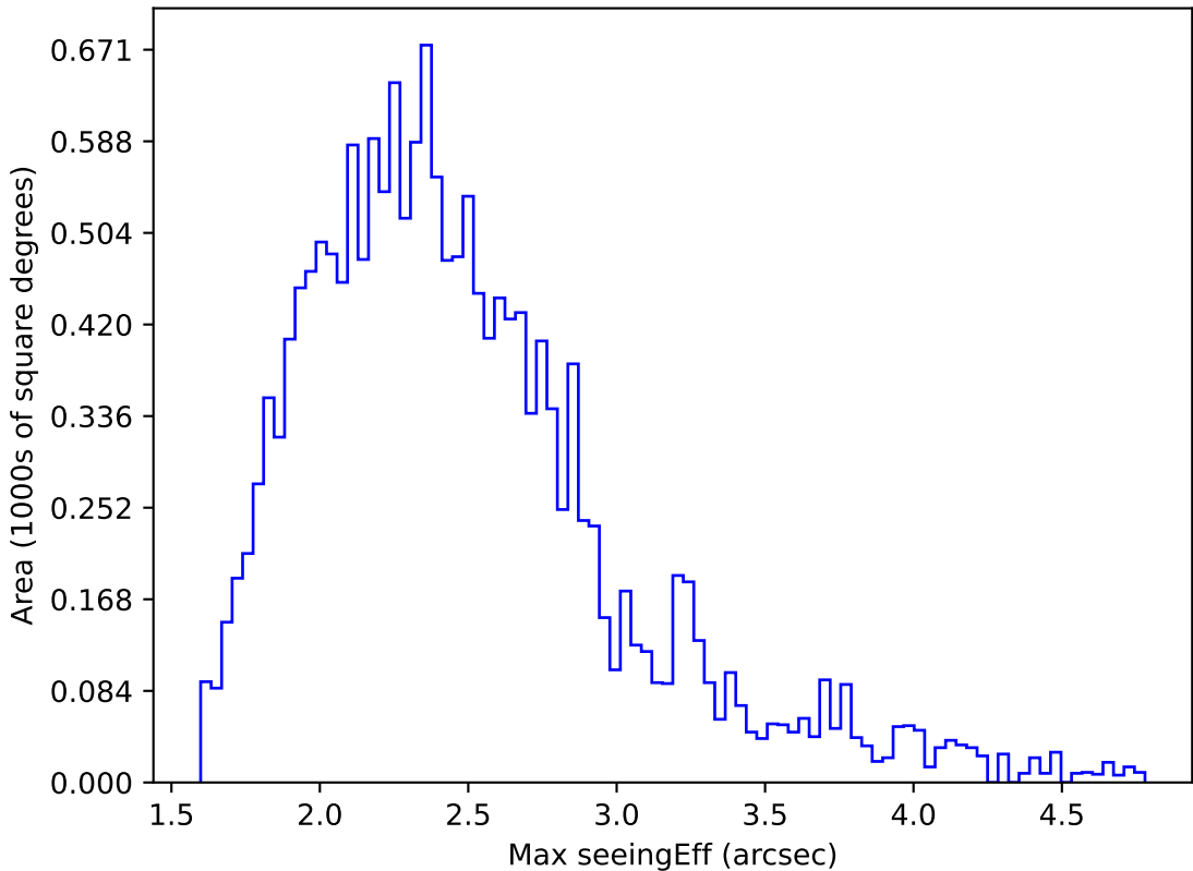
too_elab_heavy_r32_d3_griz_v3.4_10yrs WFD y band: Max seeingEff
