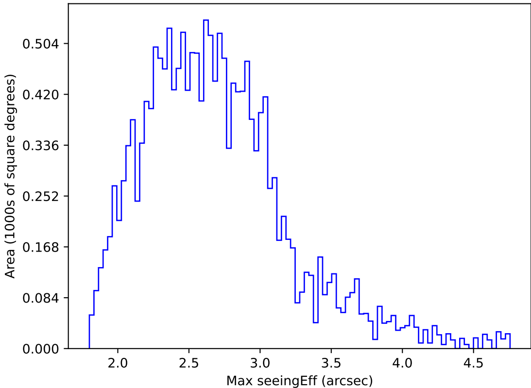
too_elab_heavy_r32_d3_griz_v3.4_10yrs WFD r band: Max seeingEff
