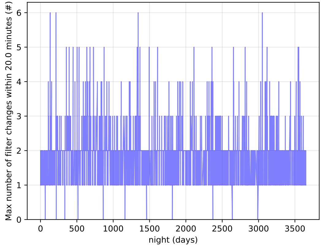
too_elab_heavy_r32_d3_griz_v3.4_10yrs Per Night: Max number of filter changes within 20.0 minutes
