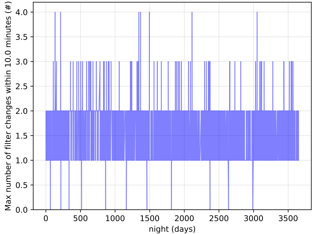
too_elab_heavy_r32_d3_griz_v3.4_10yrs Per Night: Max number of filter changes within 10.0 minutes
