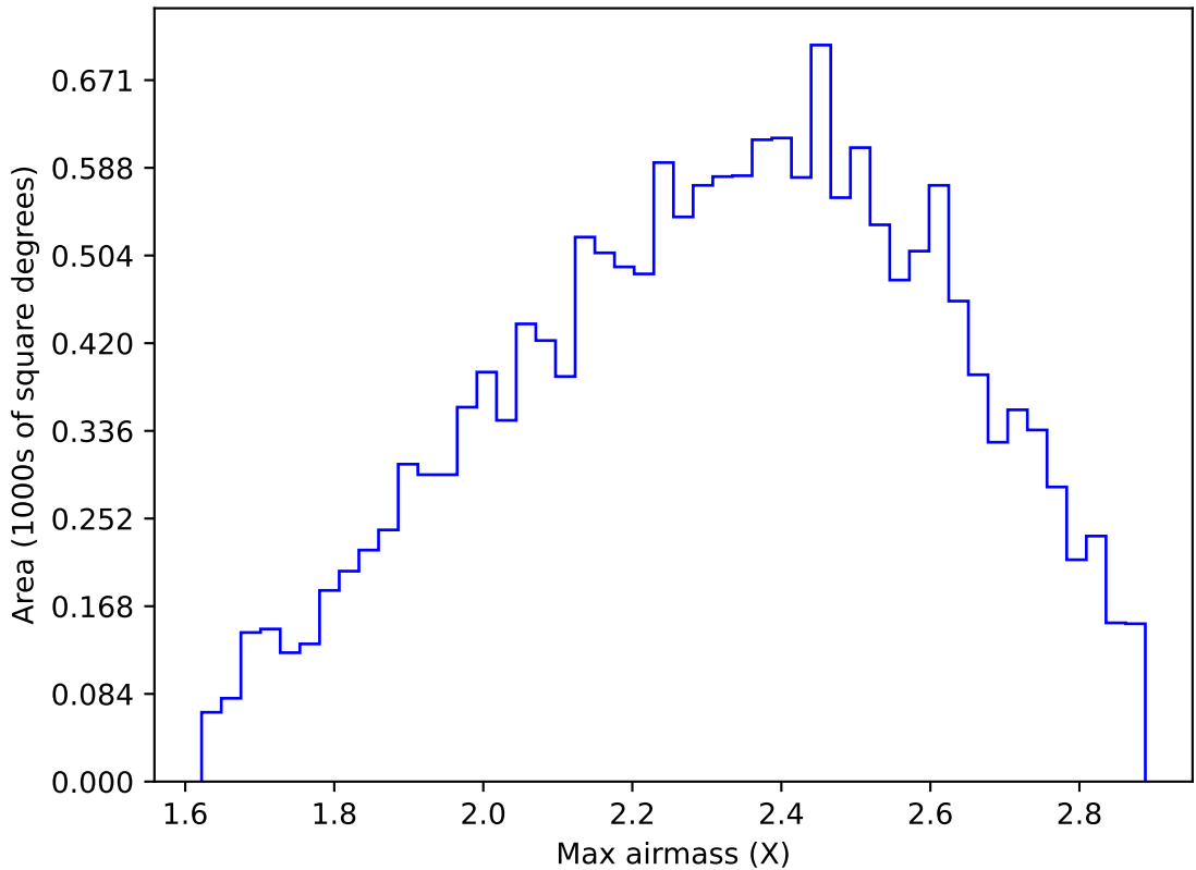
too_elab_heavy_r32_d3_griz_v3.4_10yrs WFD y band: Max airmass
