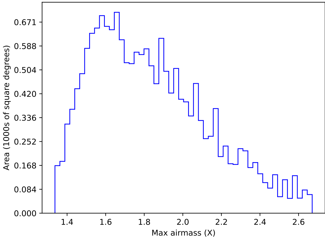
too_elab_heavy_r32_d3_griz_v3.4_10yrs WFD u band: Max airmass
