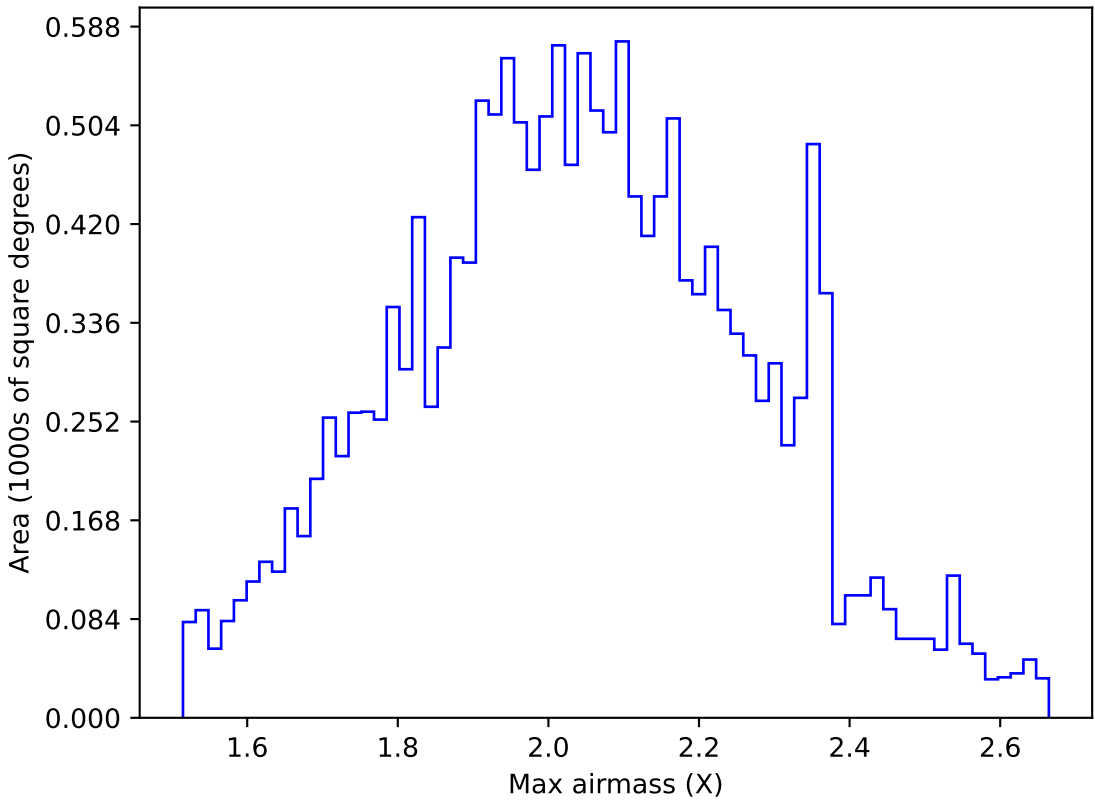
too_elab_heavy_r32_d3_griz_v3.4_10yrs WFD g band: Max airmass
