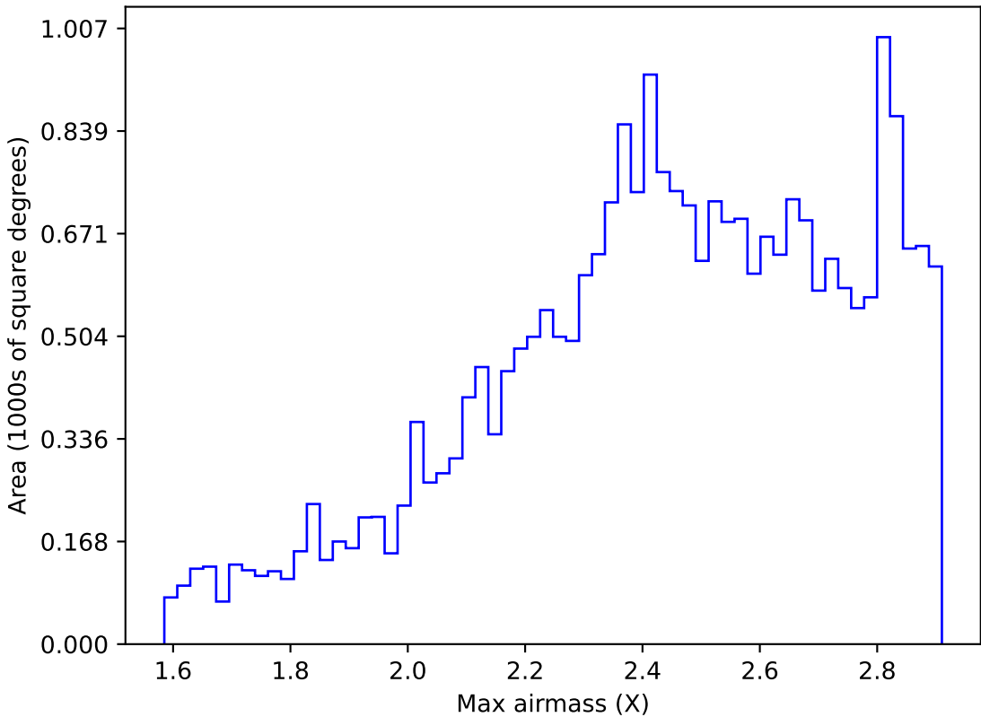
too_elab_heavy_r32_d3_griz_v3.4_10yrs All sky z band: Max airmass
