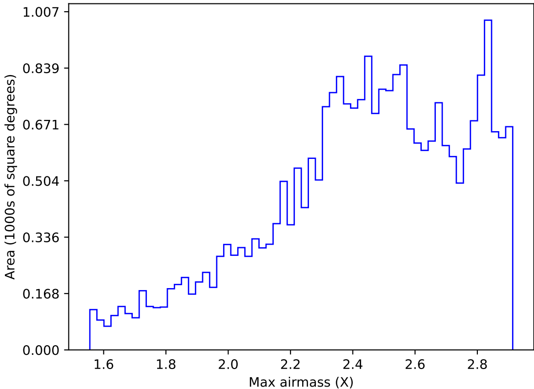
too_elab_heavy_r32_d3_griz_v3.4_10yrs All sky i band: Max airmass
