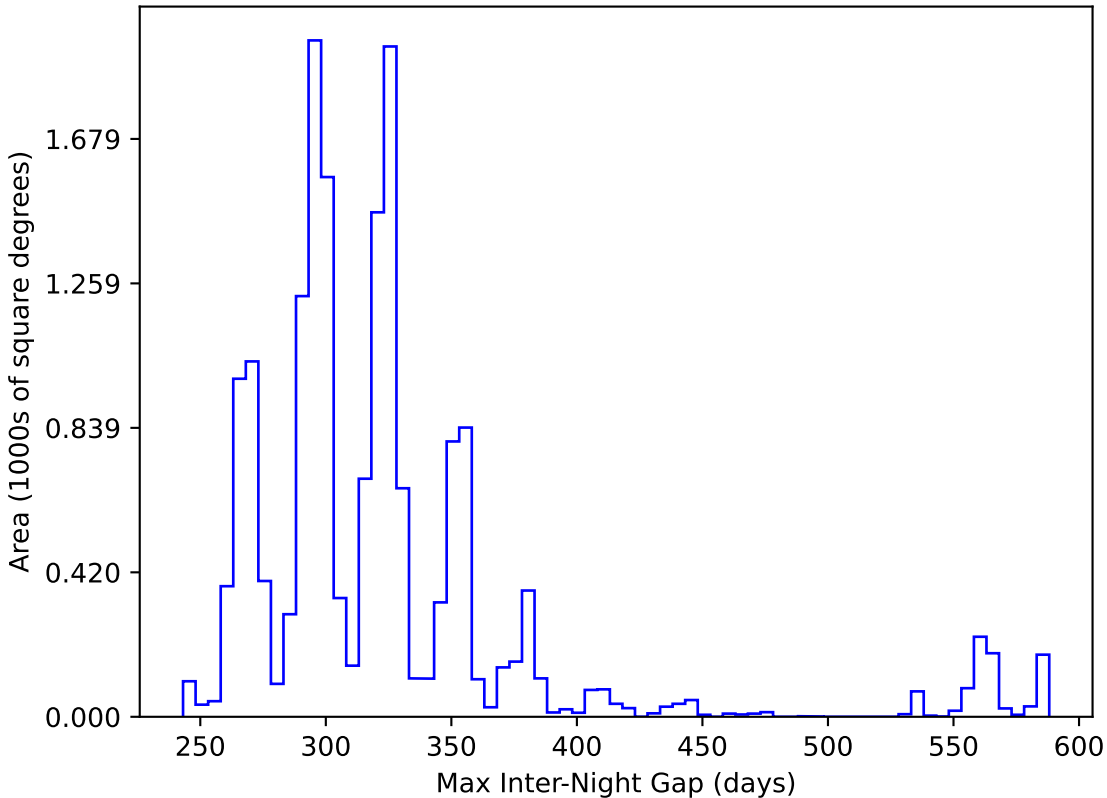
too_elab_heavy_r32_d3_griz_v3.4_10yrs WFD y band: Max Inter-Night Gap
