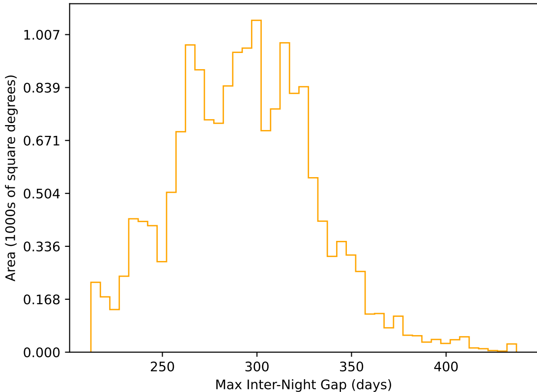
too_elab_heavy_r32_d3_griz_v3.4_10yrs WFD r band: Max Inter-Night Gap
