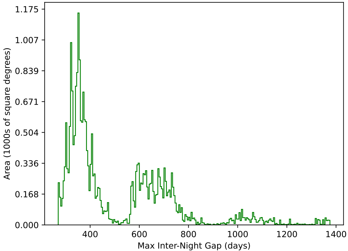
too_elab_heavy_r32_d3_griz_v3.4_10yrs All sky g band: Max Inter-Night Gap
