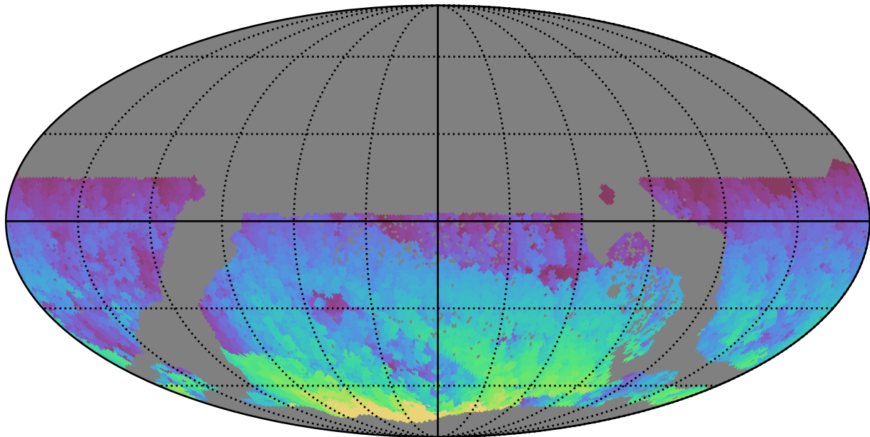
too_elab_heavy_r32_d3_griz_v3.4_10yrs WFD z band: Max HA
