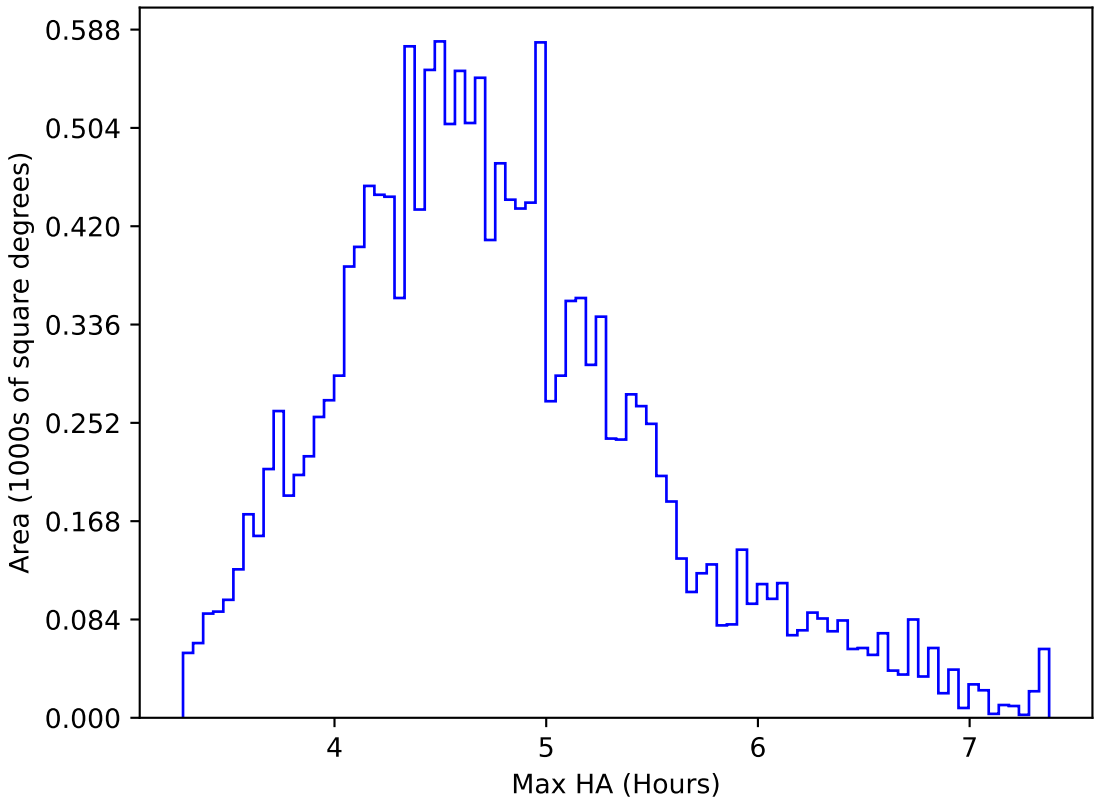
too_elab_heavy_r32_d3_griz_v3.4_10yrs WFD y band: Max HA
