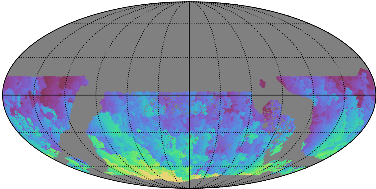
too_elab_heavy_r32_d3_griz_v3.4_10yrs WFD u band: Max HA
