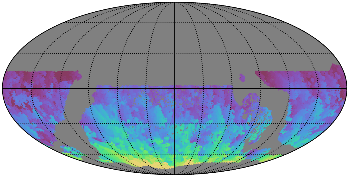
too_elab_heavy_r32_d3_griz_v3.4_10yrs WFD r band: Max HA
