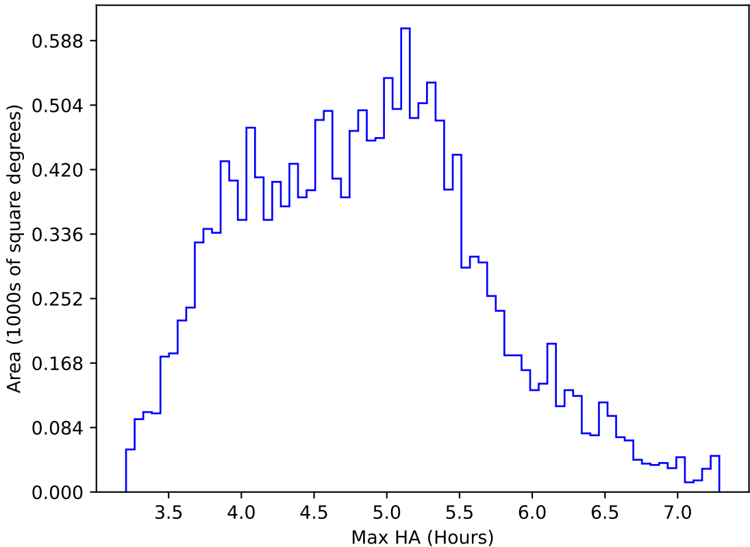
too_elab_heavy_r32_d3_griz_v3.4_10yrs WFD i band: Max HA
