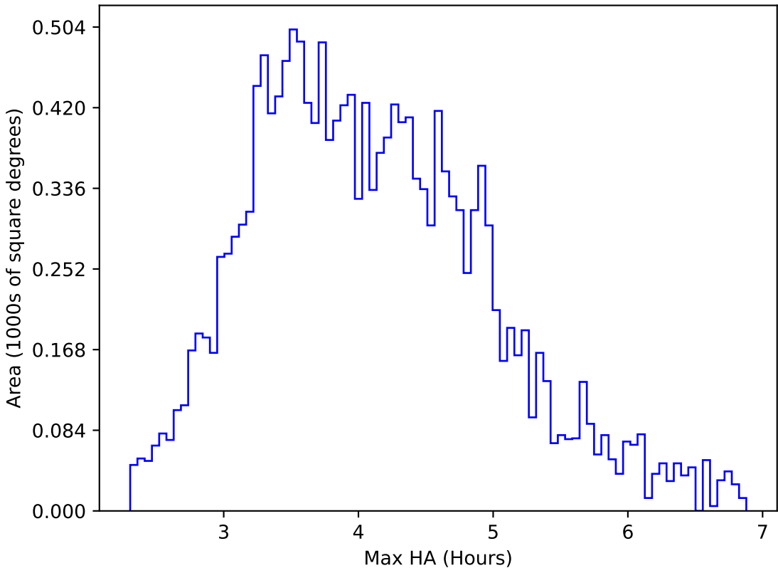
too_elab_heavy_r32_d3_griz_v3.4_10yrs WFD g band: Max HA
