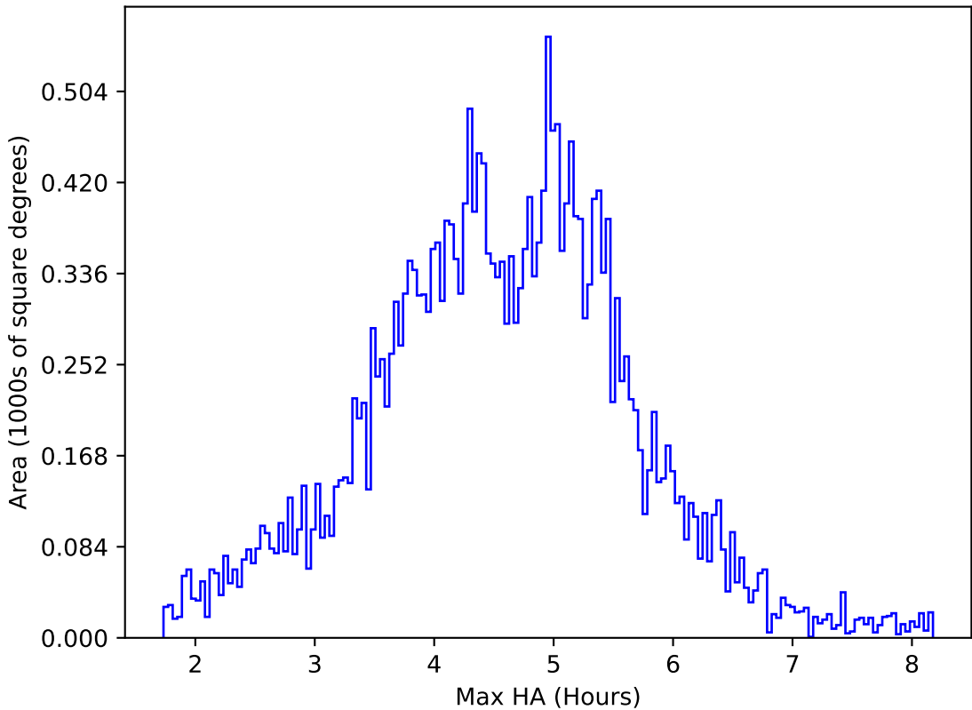
too_elab_heavy_r32_d3_griz_v3.4_10yrs All sky z band: Max HA
