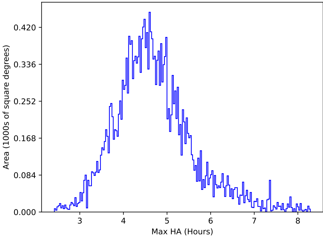
too_elab_heavy_r32_d3_griz_v3.4_10yrs All sky y band: Max HA
