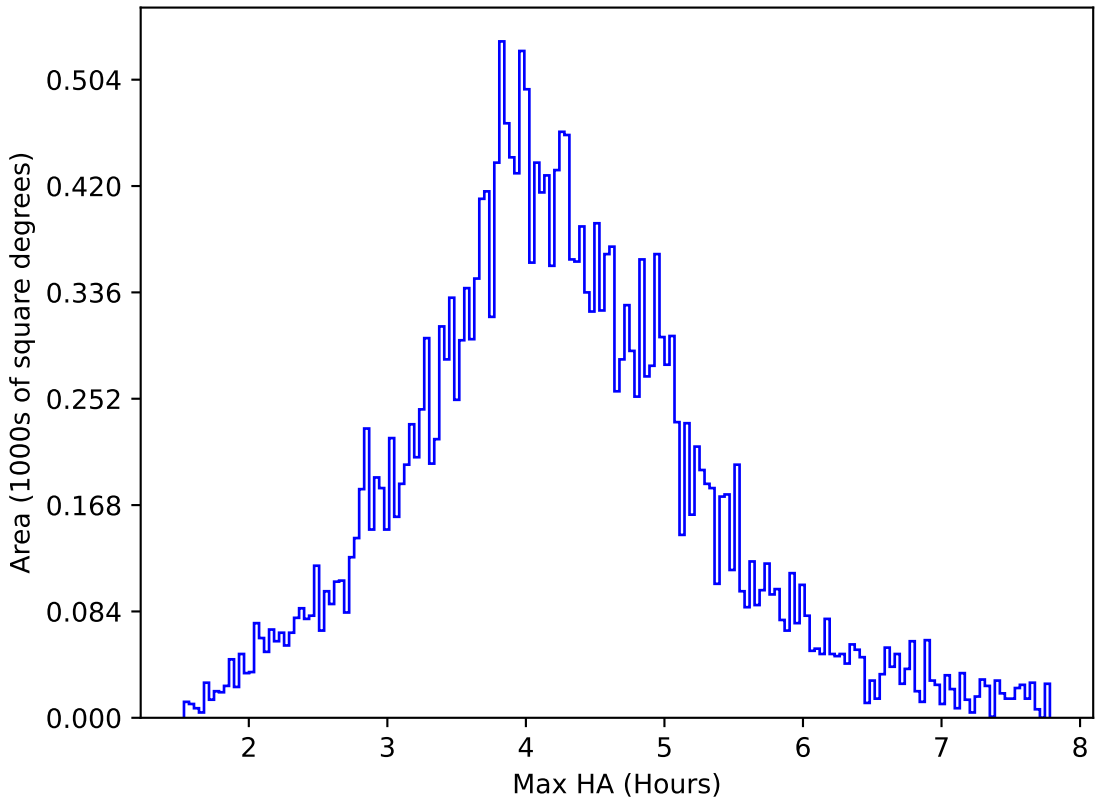
too_elab_heavy_r32_d3_griz_v3.4_10yrs All sky r band: Max HA
