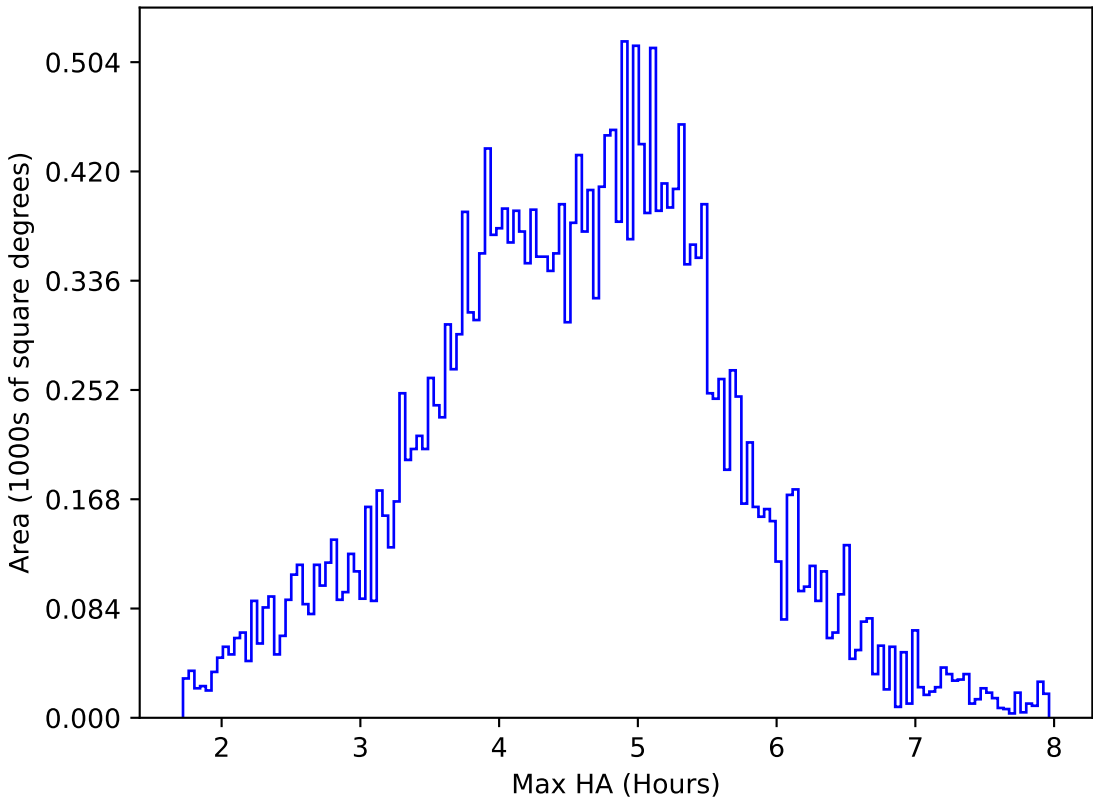
too_elab_heavy_r32_d3_griz_v3.4_10yrs All sky i band: Max HA
