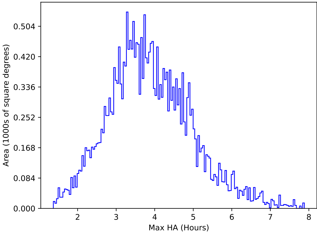
too_elab_heavy_r32_d3_griz_v3.4_10yrs All sky g band: Max HA
