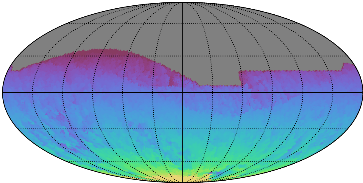
too_elab_heavy_r32_d3_griz_v3.4_10yrs All sky all bands: Max HA
