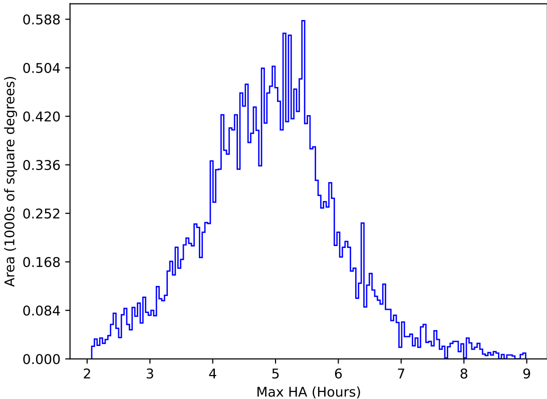
too_elab_heavy_r32_d3_griz_v3.4_10yrs All sky all bands: Max HA
