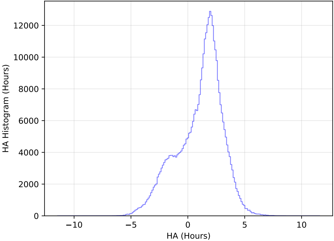
too_elab_heavy_r32_d3_griz_v3.4_10yrs WFD y band: HA Histogram
