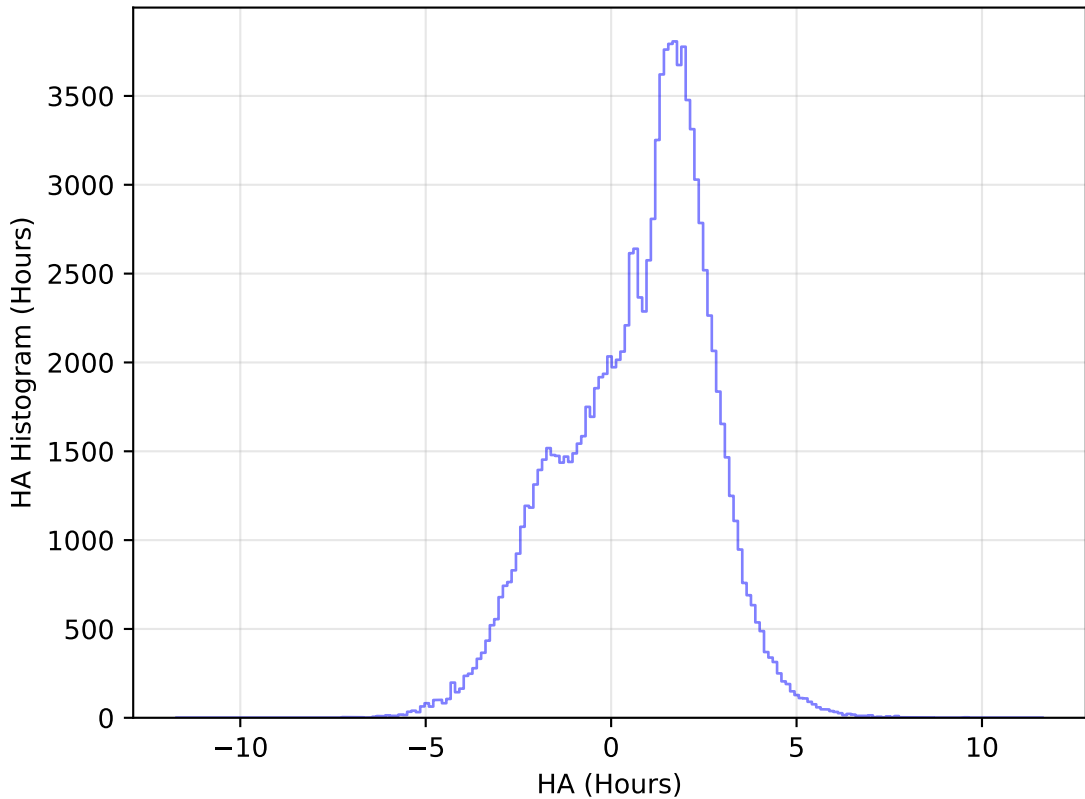
too_elab_heavy_r32_d3_griz_v3.4_10yrs WFD u band: HA Histogram
