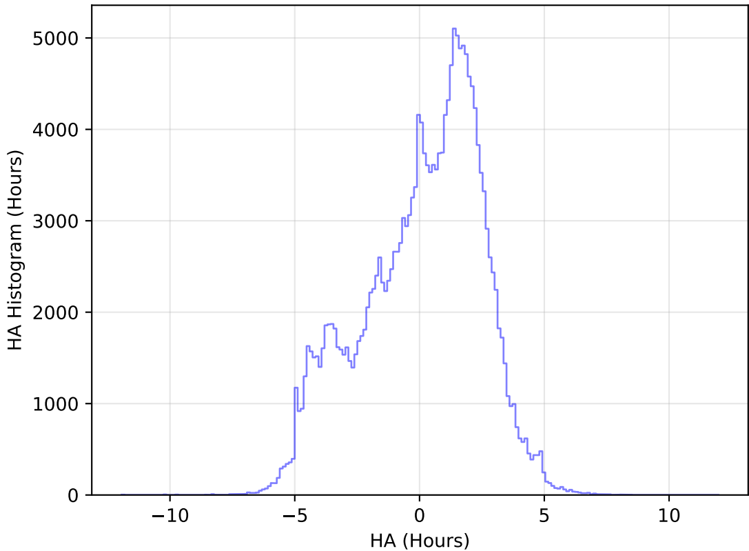
too_elab_heavy_r32_d3_griz_v3.4_10yrs WFD g band: HA Histogram
