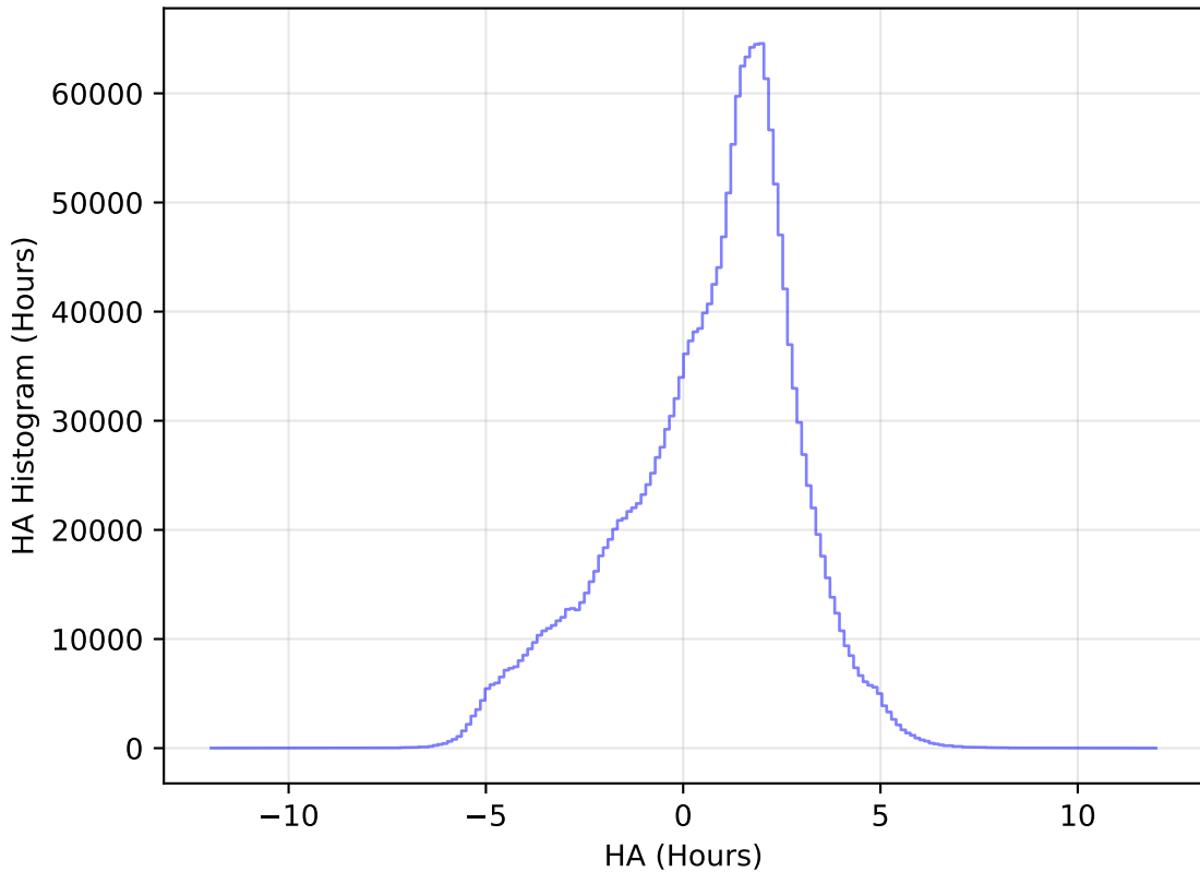
too_elab_heavy_r32_d3_griz_v3.4_10yrs WFD all bands: HA Histogram
