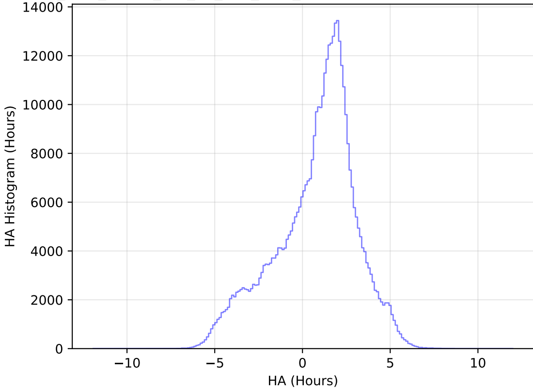
too_elab_heavy_r32_d3_griz_v3.4_10yrs All sky z band: HA Histogram
