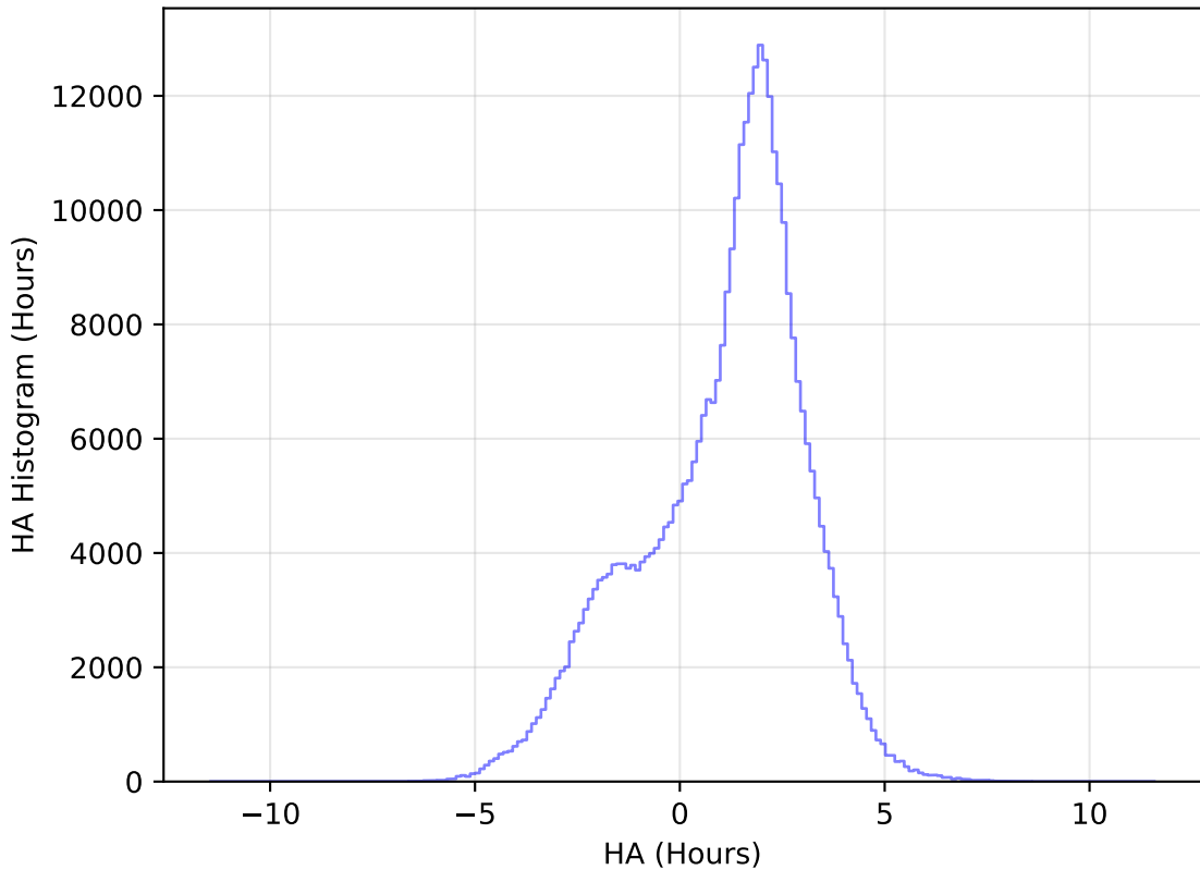
too_elab_heavy_r32_d3_griz_v3.4_10yrs All sky y band: HA Histogram
