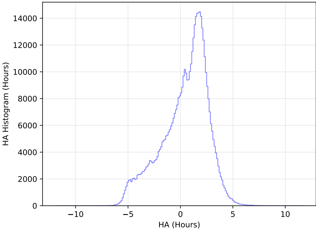
too_elab_heavy_r32_d3_griz_v3.4_10yrs All sky r band: HA Histogram
