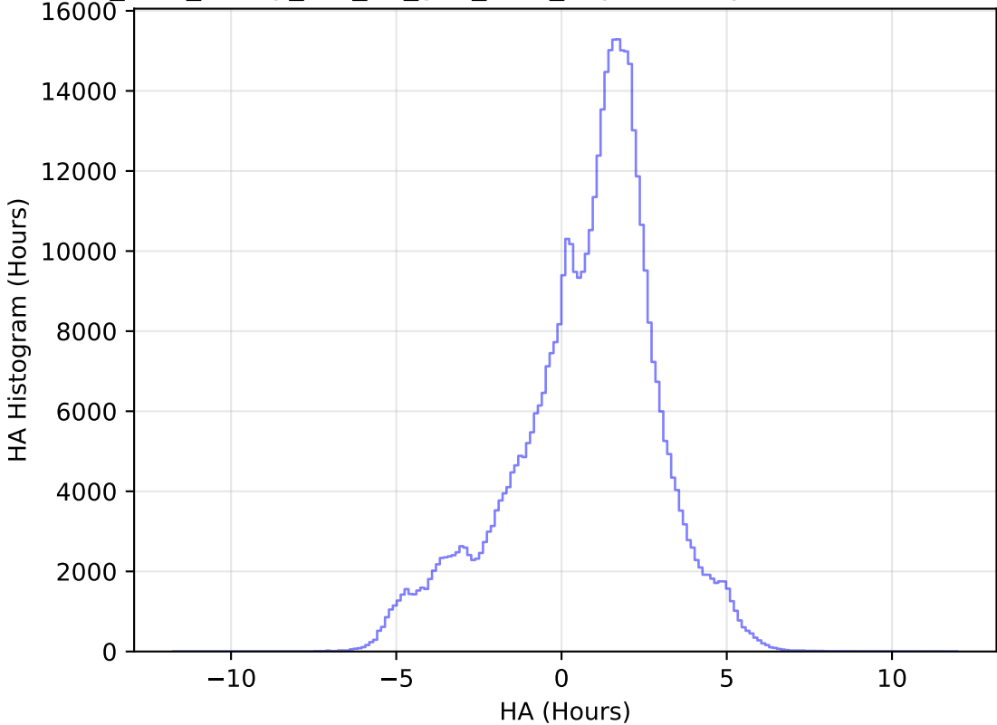
too_elab_heavy_r32_d3_griz_v3.4_10yrs All sky i band: HA Histogram
