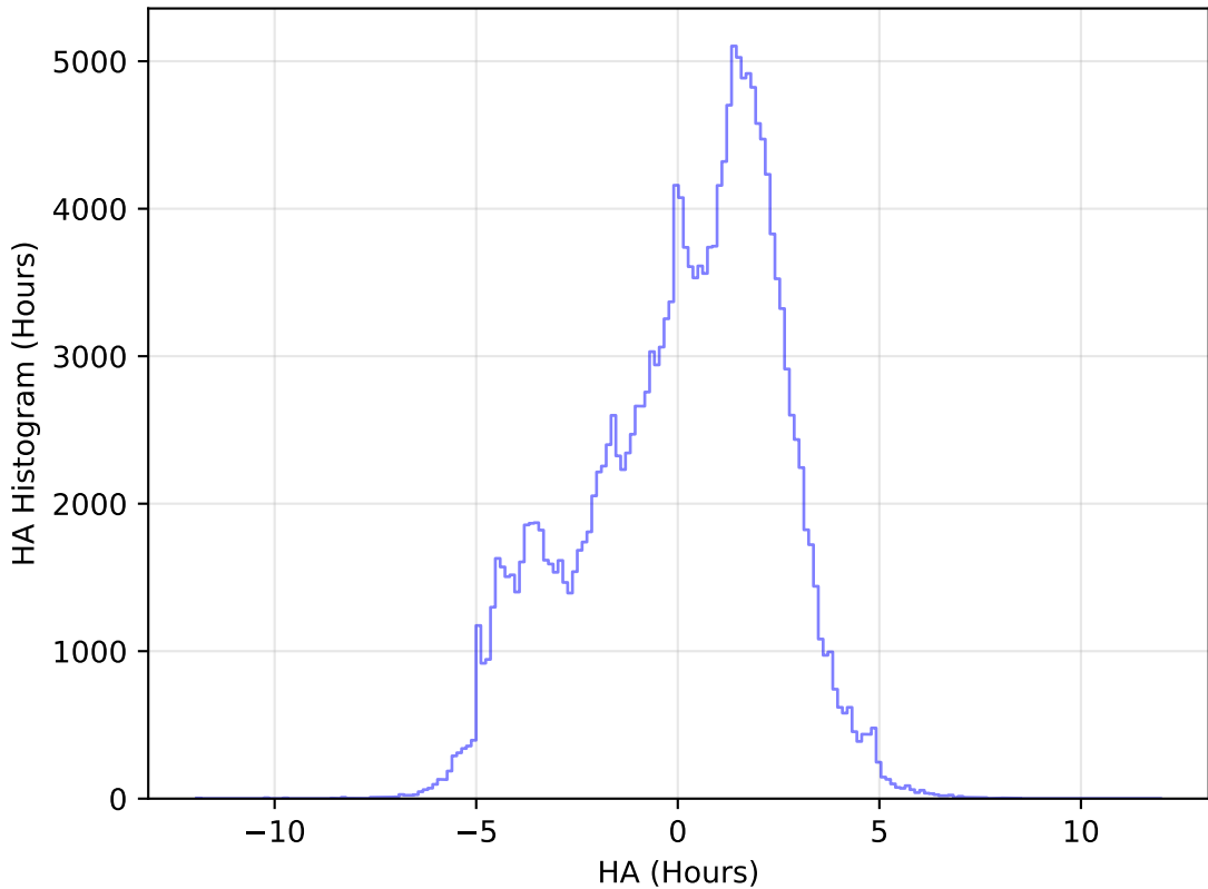
too_elab_heavy_r32_d3_griz_v3.4_10yrs All sky g band: HA Histogram
