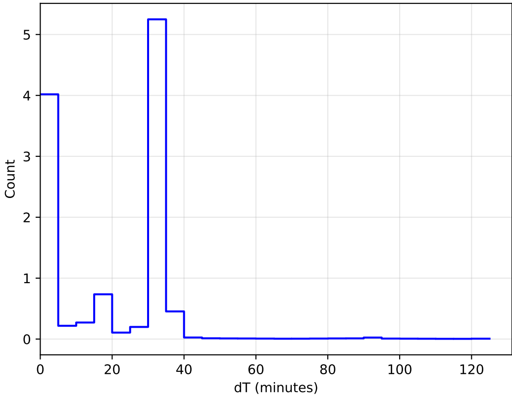
too_elab_heavy_r32_d3_griz_v3.4_10yrs WFD: DeltaT Histogram 1e6
