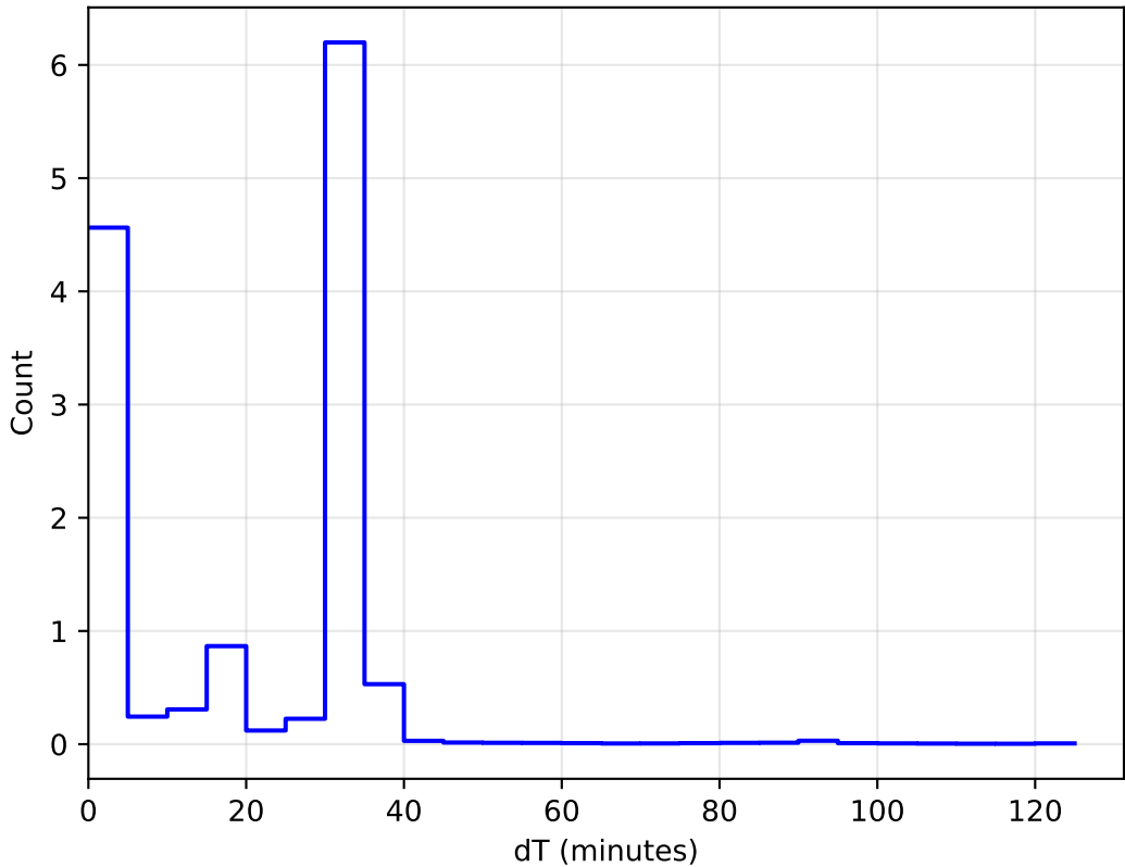
too_elab_heavy_r32_d3_griz_v3.4_10yrs All sky: DeltaT Histogram 1e6
