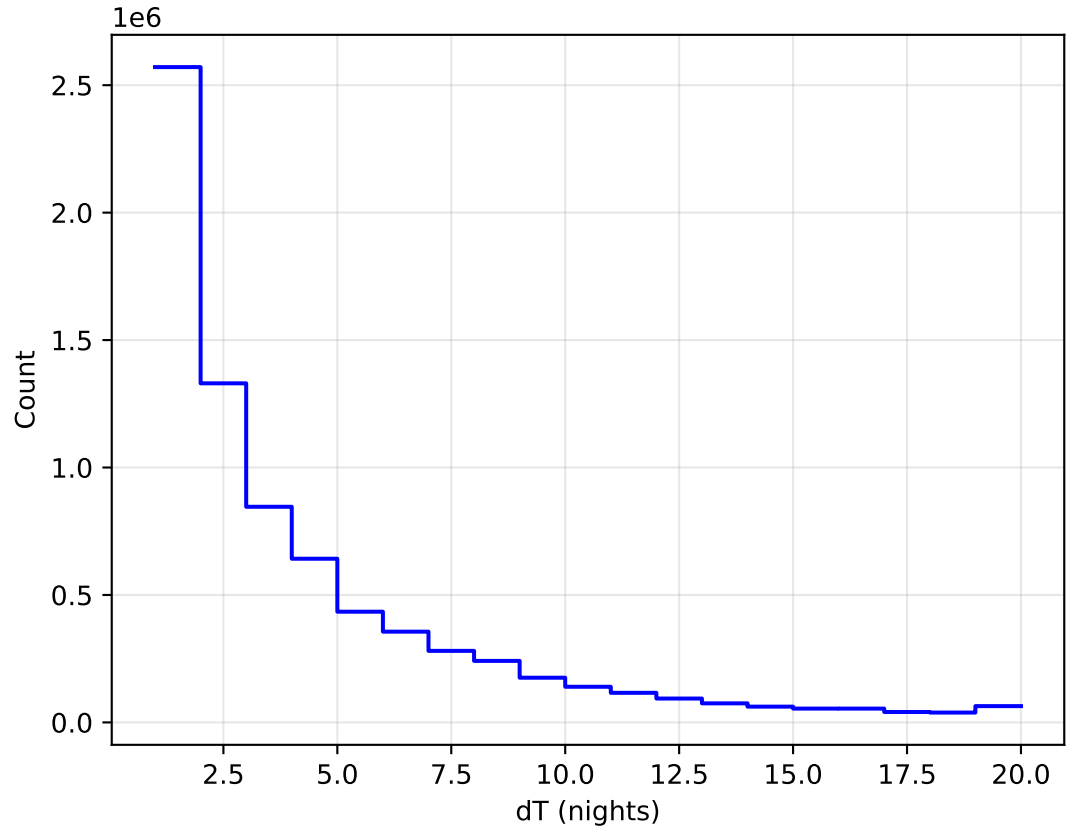
too_elab_heavy_r32_d3_griz_v3.4_10yrs WFD all bands: DeltaNight Histogram
