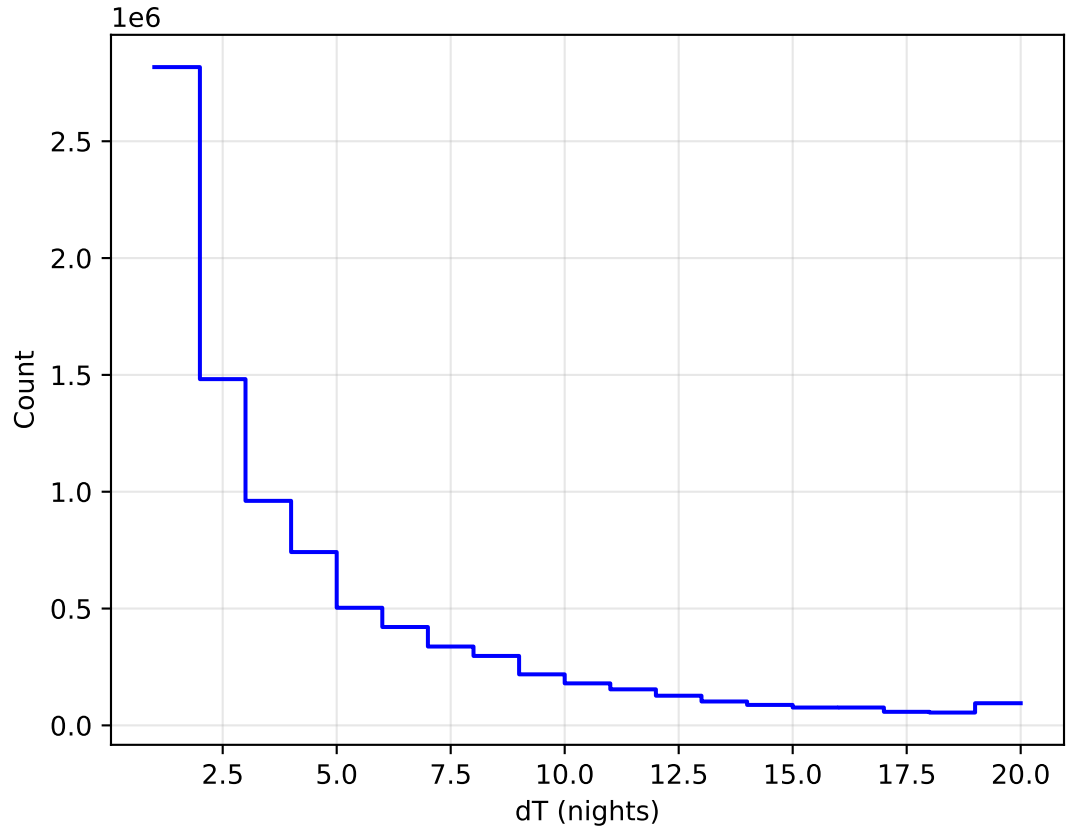
too_elab_heavy_r32_d3_griz_v3.4_10yrs All sky all bands: DeltaNight Histogram
