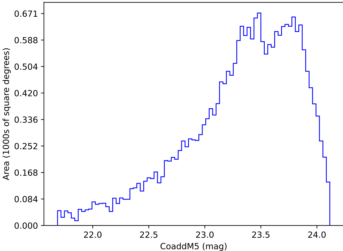
too_elab_heavy_r32_d3_griz_v3.4_10yrs Yr 3-4 y band: CoaddM5
