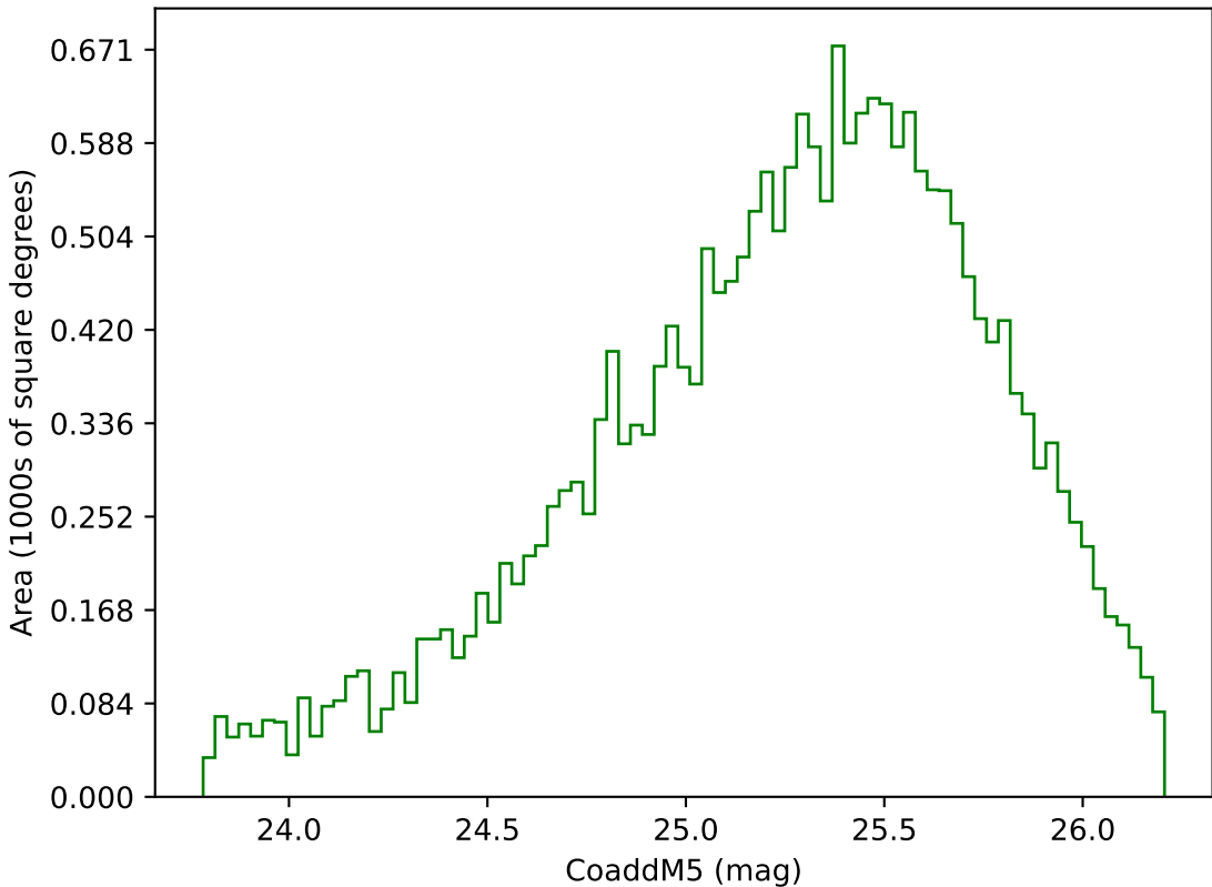
too_elab_heavy_r32_d3_griz_v3.4_10yrs Yr 3-4 g band: CoaddM5
