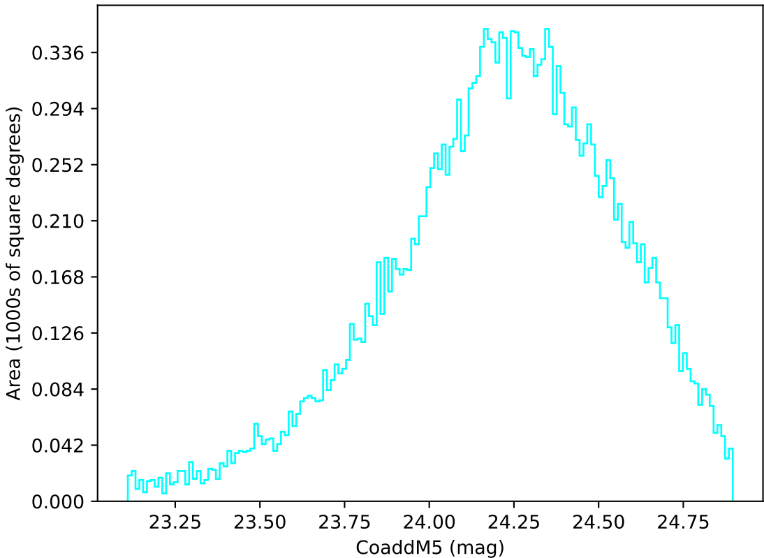
too_elab_heavy_r32_d3_griz_v3.4_10yrs Yr 1 u band: CoaddM5
