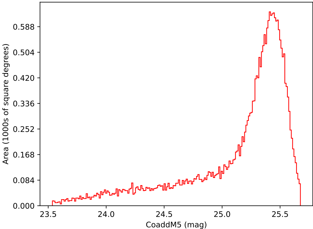
too_elab_heavy_r32_d3_griz_v3.4_10yrs Yr 1 i band: CoaddM5
