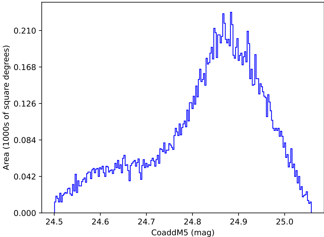
too_elab_heavy_r32_d3_griz_v3.4_10yrs WFD y band: CoaddM5
