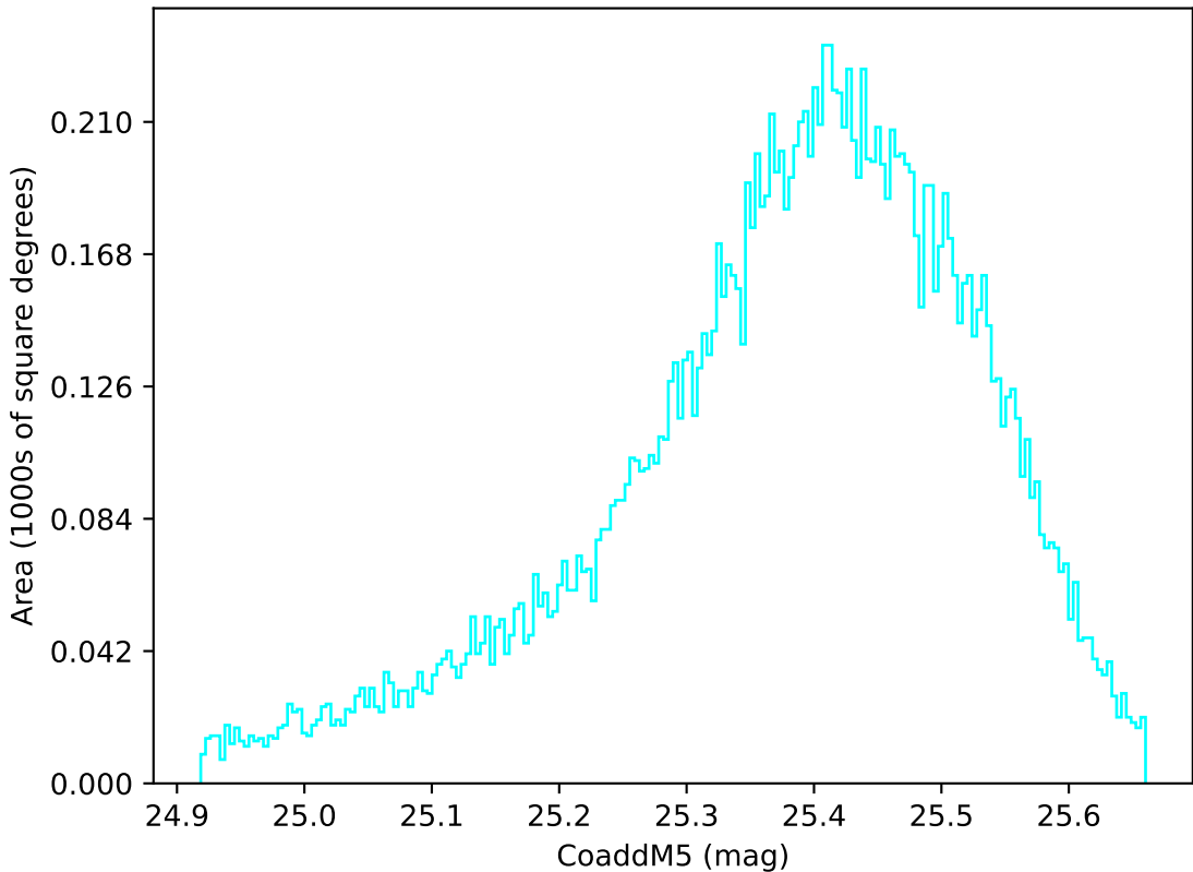
too_elab_heavy_r32_d3_griz_v3.4_10yrs WFD u band: CoaddM5
