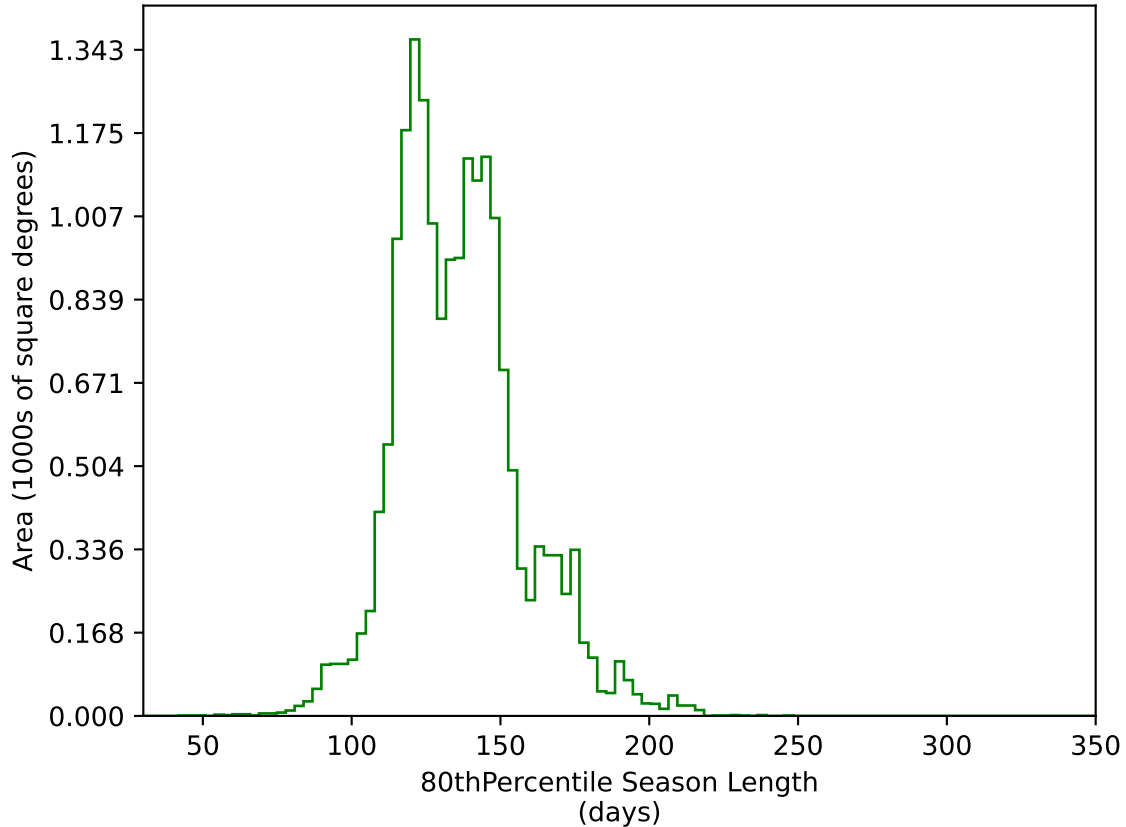
too_elab_heavy_r32_d3_griz_v3.4_10yrs WFD g band: 80thPercentile Season Length
