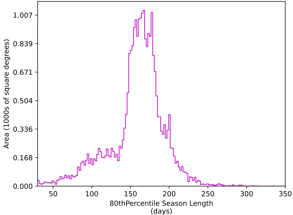
too_elab_heavy_r32_d3_griz_v3.4_10yrs All sky z band: 80thPercentile Season Length
